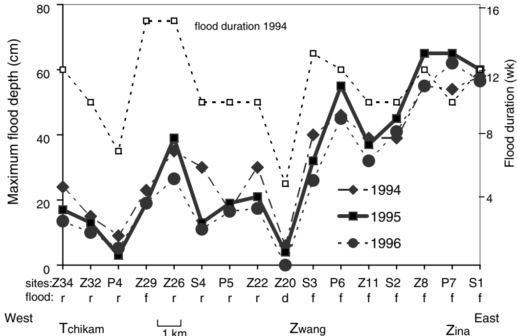
Figure 2. Maximum flood depth and flood duration in the transect Zina–Zwang–Tchikam. For position, see also Figure 1. Flood situation: f: flooded (before and after 1994), r: reflooded from 1994 onwards, d: dry (before and after 1994).
